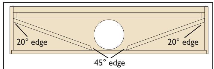
Fig. 1 - Cross-section
