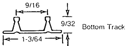
Nylon roller Extra nylon rollers are available.
