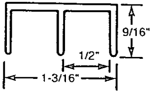
Channel for use as upper guide
